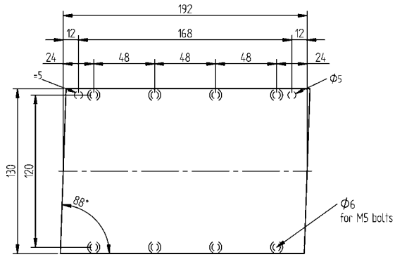
Magnetplate 192mm
