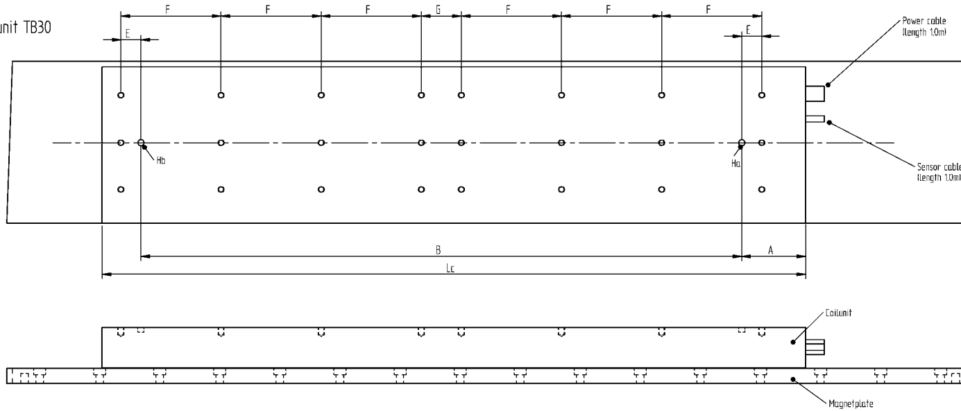
Dimensions of Coilunits
