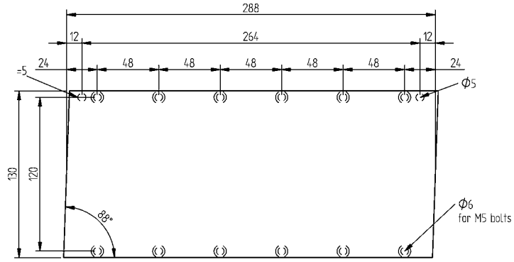
Magnetplate 288mm
